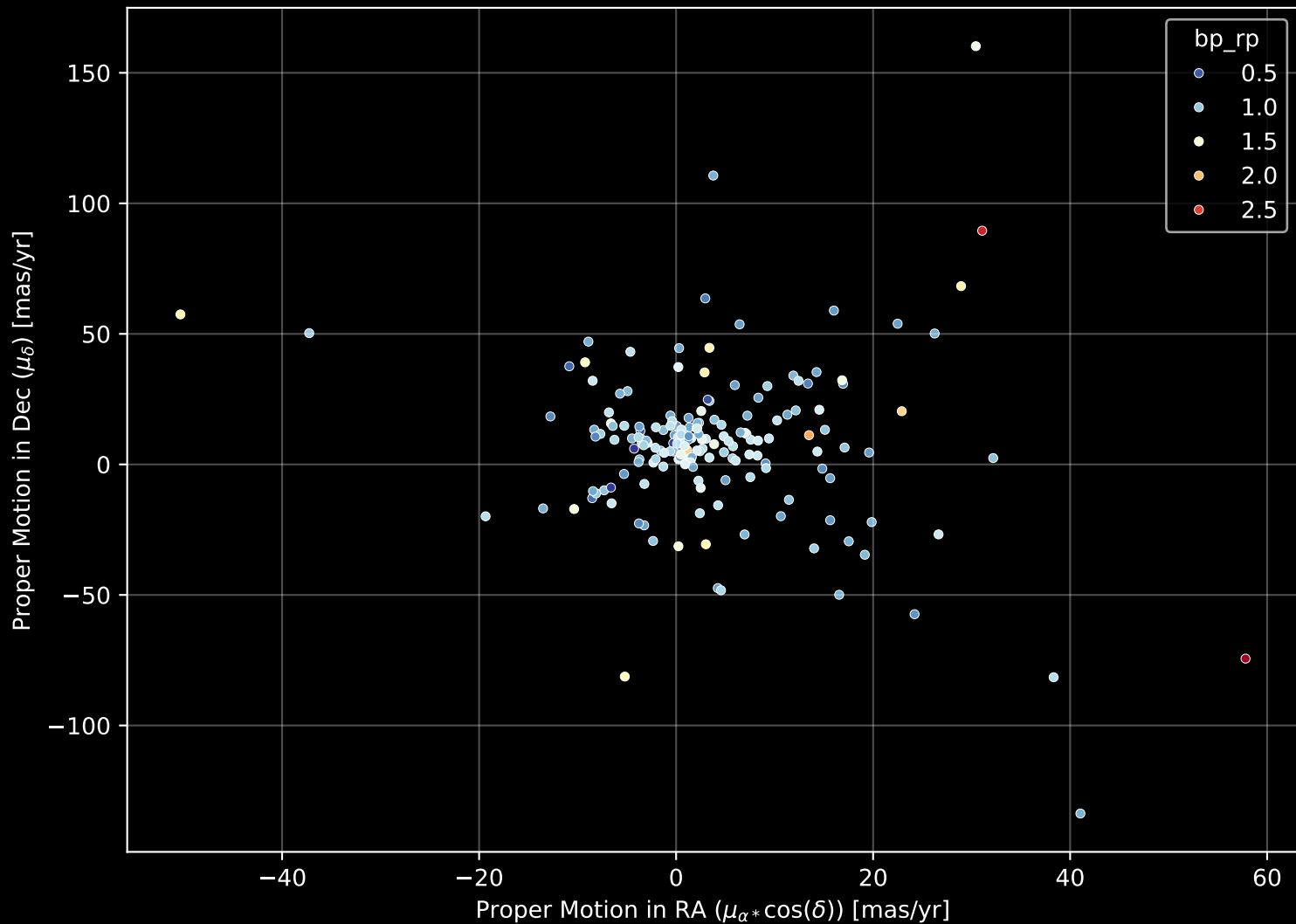
APOGEE DR17 Field: [267-30-O_TESS] Proper Motion Diagram (n= 184)
