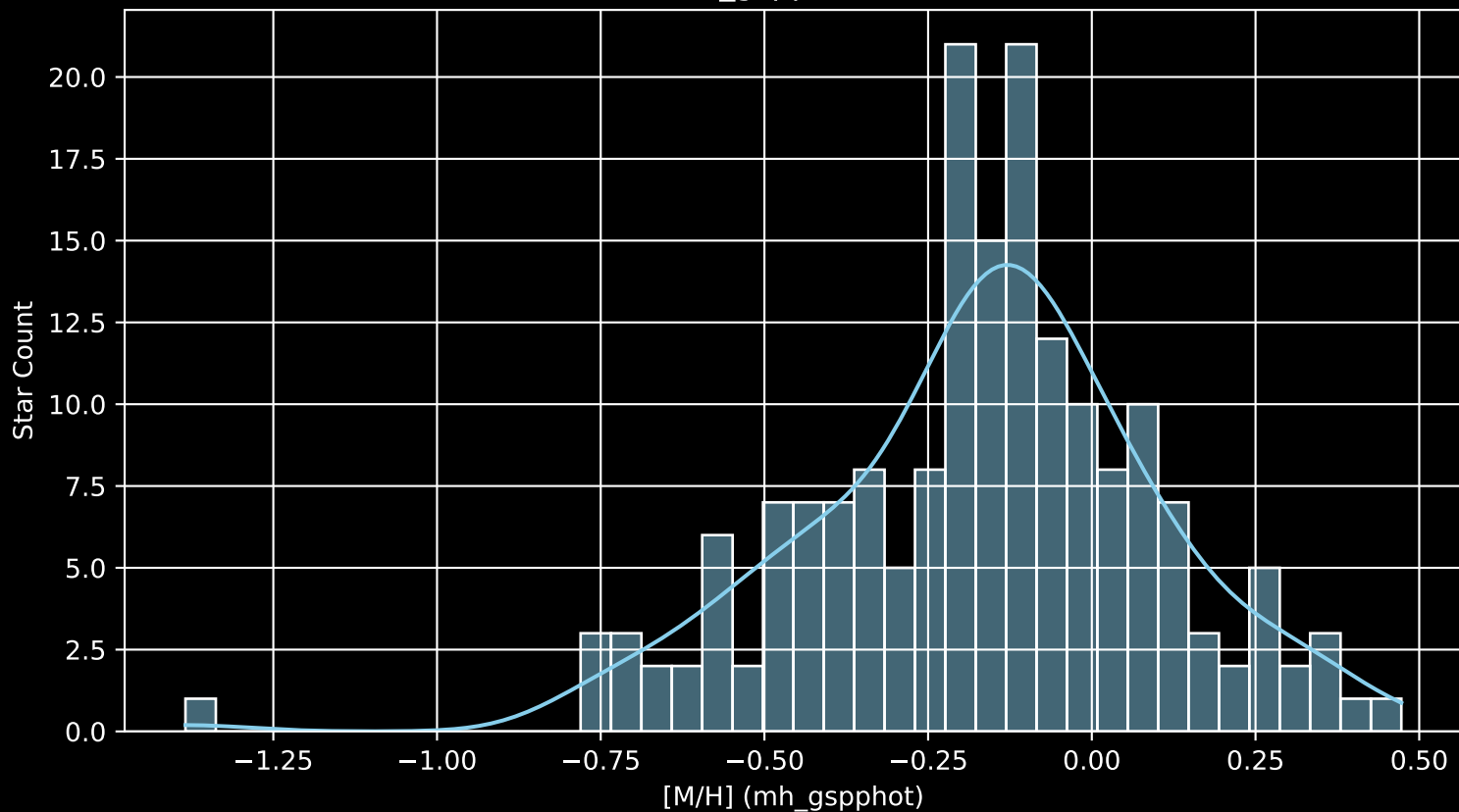
APOGEE DR17 Field: [267-30-O_TESS [M/H] (mh_gspphot) (n= 182)
