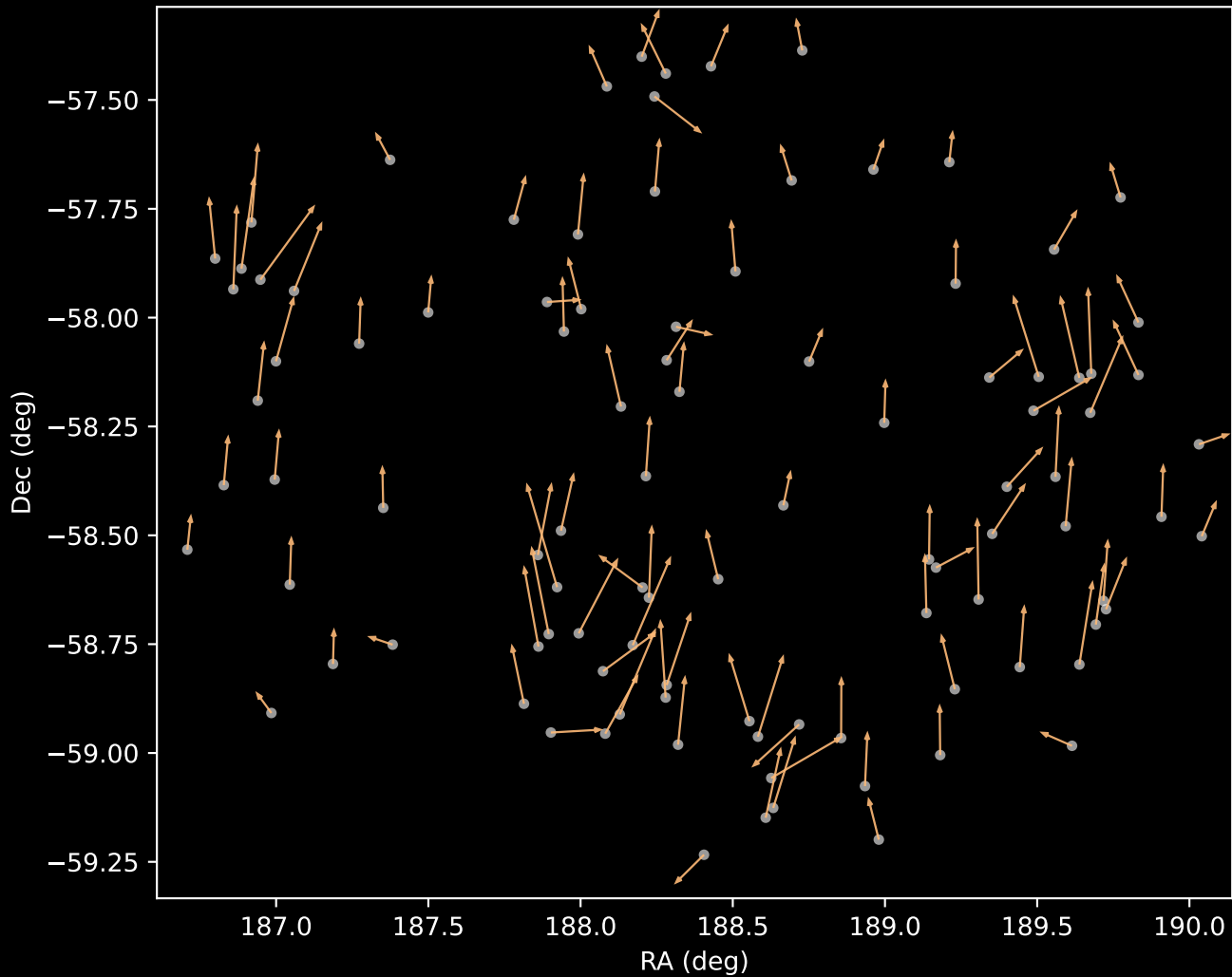
APOGEE DR17 Cluster 3 Proper Motion Vectors (n=101)
