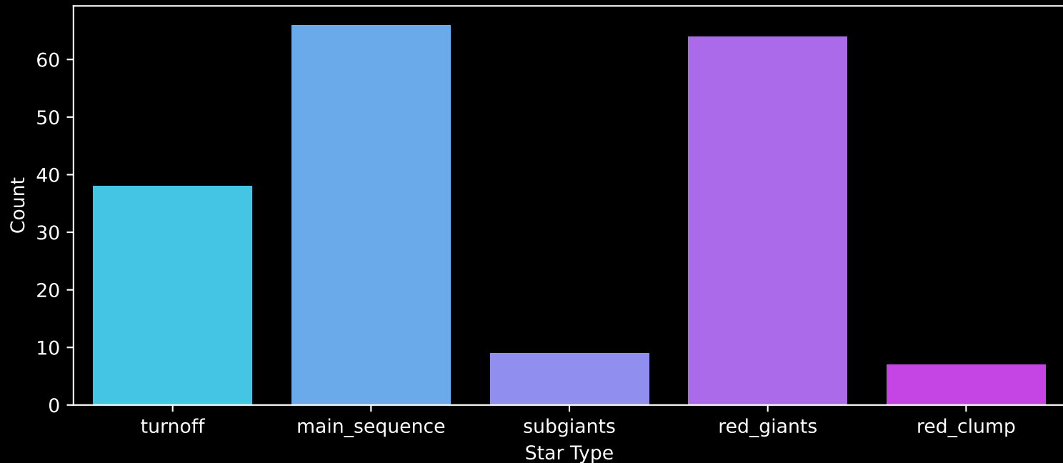
APOGEE DR17 Field: [267-30-O_TESS] Count plot of Star Type
