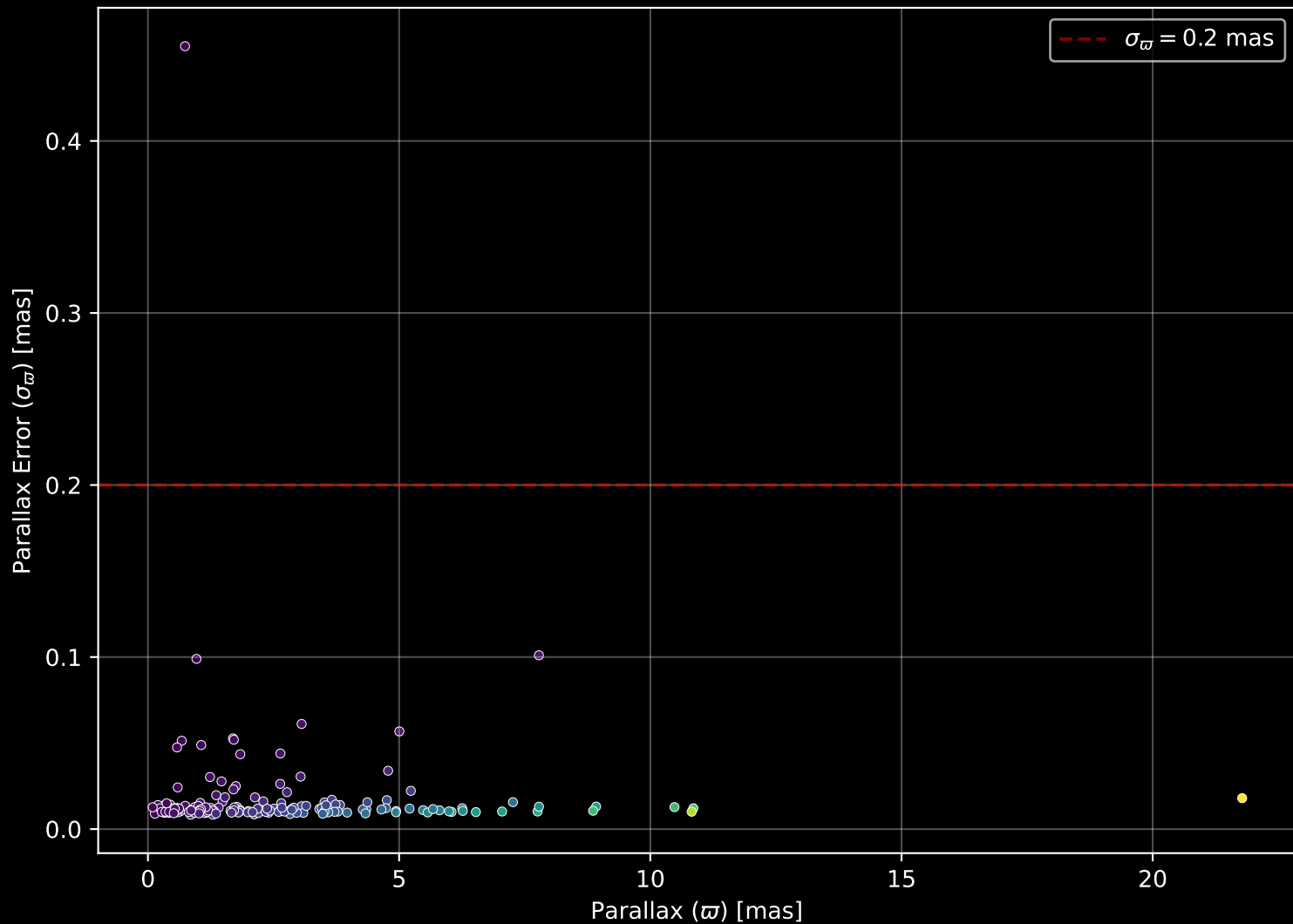
APOGEE DR17 Field: [267-30-O_TESS] Parallax Quality (n= 184)
