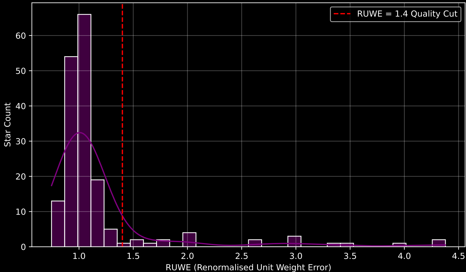
GAPOGEE DR17 Field [267-30-O_TESS] RUWE Distribution (n= 177)
