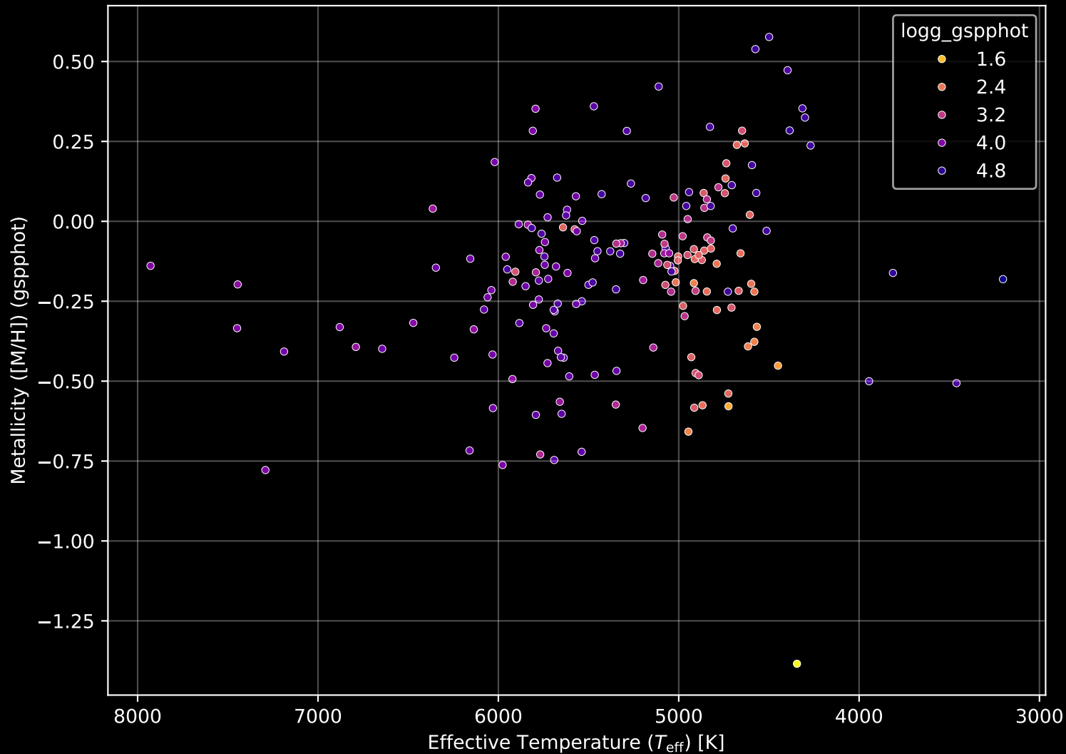
APOGEE DR17 Field: [267-30-O_TESS] Stellar Population Parameters (n= 184)
